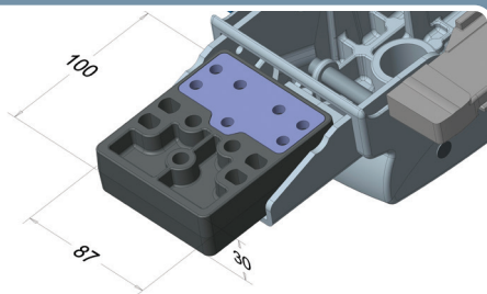
Staffa compensatrice con piastrina filettata Compensator bracket with threaded plate
