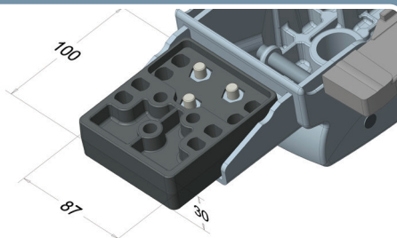
Staffa compensatrice con dadi Compensator bracket with nuts
